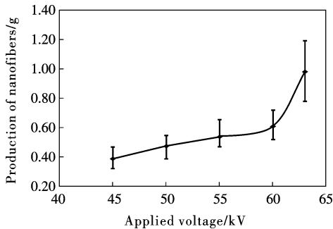
Fig. 4 Curve of throughput of nanofibers vs applied voltage by electrospinning for 30 min (The concentration of PEO solution is 14% and the electrode distance is 35 cm)
