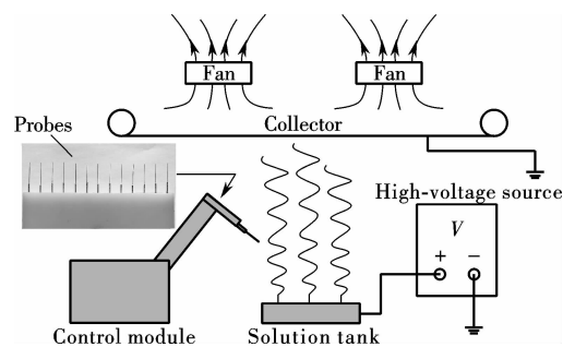
Fig. 1 Schematic diagram of TIE setup
