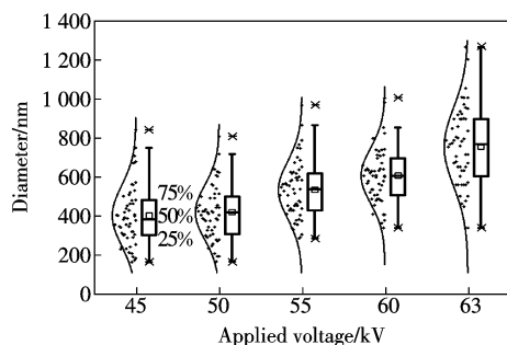
Fig. 7 Diameter distribution of the electrospun nanofibers under different applied voltages (The concentration of PEO solution is 14% and the electrode distance is 35 cm)
